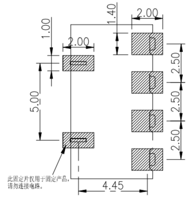
RECOMMENDED PCB LAYOUT TOP VIEW (.XX±0.05)
